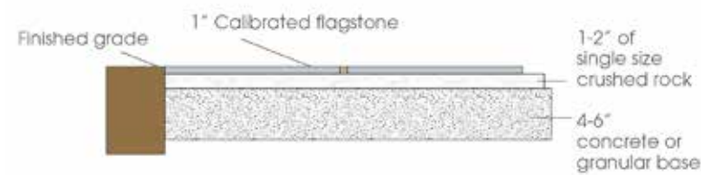
Typical cross-section
